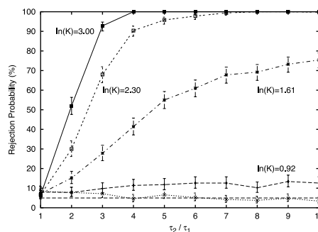
FIGURE 2 Rejection probability. The probability of rejecting the null hypothesis of detailed balance against the ratio of open times \tau_2/\tau_1 is shown for different values of \ln(K) where K is the ratio of transition rates in clockwise and counterclockwise direction. The line at the bottom corresponds to a value of \ln(K) = 0.22 . To calculate the rejection probability, we simulated 500 recordings for each \tau_2/\tau_1 and \ln(K) . The number of simulated dwell times per record ranges from 31,149 to 24,441, depending on the value of \ln(K) .
