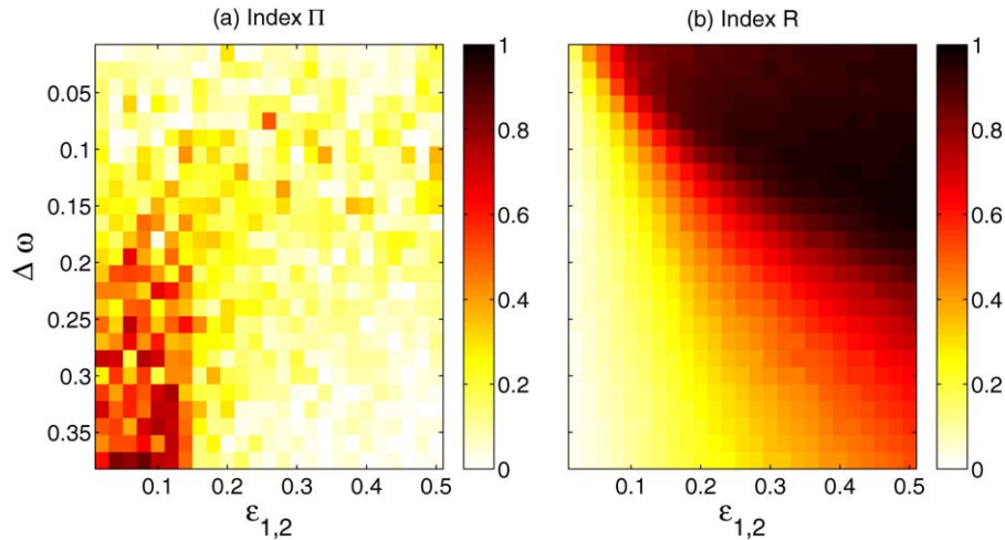
Fig. 4. (a) Index \Pi (cf. Eq. (16)) for a coupled stochastic Roessler system depending on the bidirectional coupling \varepsilon_{1,2} and frequency mismatch \Delta\omega . (b) Values of the corresponding synchronization index R (cf. Eq. (10)). The upper right corner shows high values of R , strongly indicating a preferred value of the phase difference. In the area with high synchronization index R , the index \Pi quantifying a preferred direction of phase jumps is close to 0. The high values of \Pi in the lower left area can be neglected since no phase synchronization is detected by the index R .
