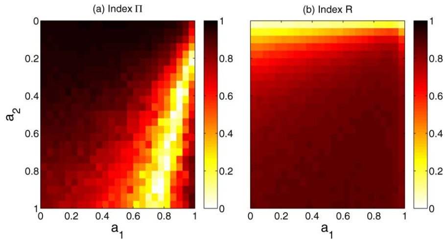
Fig. 5. (a) Index \Pi (cf. Eq. (16)) for the transfer function system depending on parameters a_1 and a_2 . (b) Values of the corresponding synchronization index R (cf. Eq. (10)). If a_2 exceeds a value of 0.2, independent of a_1 , high values for the synchronization index are estimated leading erroneously to conclusion of phase synchronization. The index \Pi indicating a preferred direction of phase jumps is close to one in the area of high values of R . Only in a small area for a_1 between 0.6 and 0.8, the index \Pi is close to zero.
