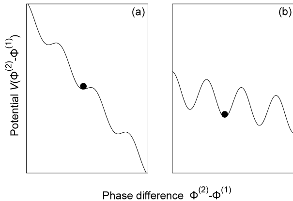
Fig. 3. Washboard potential of the phase difference for two different parameter choices. In (a) a low coupling strength and a high frequency mismatch between the Roessler systems is chosen. In (b) the frequency mismatch is chosen to be low compared to the high coupling. The stochastic influence may lead to jumps of the phase difference in both directions with almost the same probability in (b). In contrast, phase jumps in the positive horizontal direction are more likely in (a).
