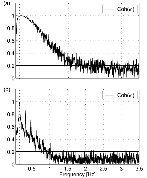
Fig. 2. Coherence between the x -component of a Roessler oscillator and its propagated signal u (a) and coherence between the x_1 - and x_2 -components of a bidirectionally coupled stochastic Roessler system (b). The dotted vertical line indicates the oscillation frequency of the input oscillator in (a) and the common frequency of the synchronized oscillators in (b). Since in both figures coherence exceeds the critical values for a 1%-significance level, given by the solid, horizontal line, a linear relationship is strongly indicated. A differentiation between both classes of dynamic systems is impossible by just applying coherence analysis.
