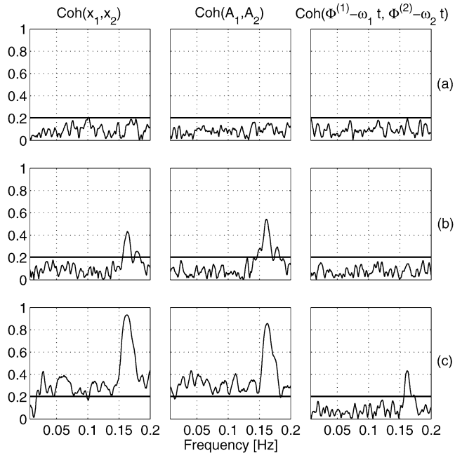
Fig. 6. Coherences estimated between the components x_1 and x_2 , the amplitudes of the analytic signal A_1 and A_2 as well as coherence between the phase fluctuations for three coupling strengths \varepsilon_{1,2} of a bidirectionally coupled stochastic Roessler system. The 1%-significance level is given by the solid horizontal lines. (a) For a low coupling strength of \varepsilon_{1,2} = 0.008 , no significant coherences are detected in neither of these coherence spectra. (b) For \varepsilon_{1,2} = 0.024 , significant coherences are observed for the x -components and the amplitudes at the oscillation frequency \omega/2\pi \approx 0.16 Hz, while the phase fluctuations are still not coherent. (c) Coherences for a coupling strength of \varepsilon_{1,2} = 0.084 . All three coherence spectra show a significant peak at the oscillation frequency. The coherence between the phase fluctuations is exclusively significant at the oscillation frequency. Additionally, coherence between the components as well as coherence between the amplitudes is significant in the low frequency range.
