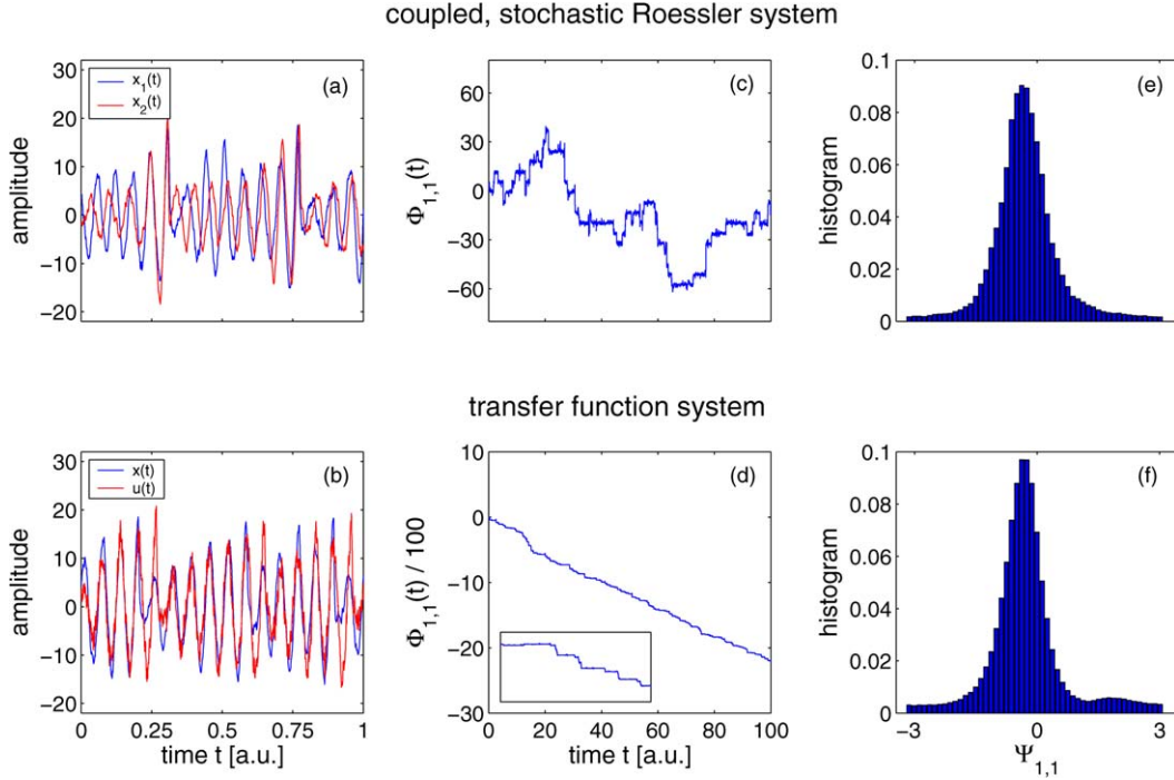
Fig. 1. Time series of a coupled stochastic Roessler system (a) and of the considered transfer function model ( \tau = 64 ) (b). Phase difference \Phi_{1,1} for the coupled stochastic Roessler system (c) and for the transfer function model (d). The small subplot in (d) shows a section of the phase difference of two time units duration more closely. Considering the temporal evolution of the phase differences \Phi_{1,1} , rapid phase changes in one direction are preferred for the transfer function model. For the coupled stochastic Roessler system, phase jumps in both directions occur with almost the same frequency in this example. Corresponding normalized histograms of \Psi_{1,1} in (e) and (f). Even if both systems possess a different dynamic behavior, a preferred value of \Psi_{1,1} is taken for both. A differentiation between both classes of dynamics is impossible by just applying phase histogram analysis.
