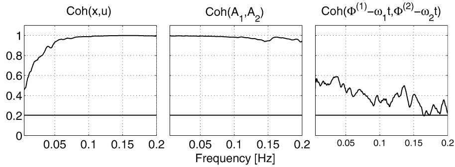
Fig. 7. Coherences between the components x and u , between the amplitudes A_1 and A_2 as well as coherence between the phase fluctuations for the transfer function system. The 1%-significance level is given by the solid horizontal lines. All three coherence spectra are highly significant over a broad frequency range. Especially a significant coherence between the phase fluctuations is detected in the entire low frequency band. This is in contrast to the coupled stochastic Roessler system.
