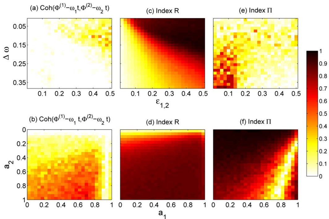
Fig. 8. Averaged coherence values between the phase fluctuations (a), values of the phase synchronization index R (c), and values of the index \Pi quantifying direction of phase jumps (e) for the coupled stochastic Roessler system. Averaged coherence values between phase fluctuations (b), values of the phase synchronization index R (d), and values of the index \Pi (f) for the transfer function system. For a high value of the synchronization index R , combination of coherence applied to the phase fluctuations and the direction of phase jumps allows for specific conclusions about the underlying dynamics.
